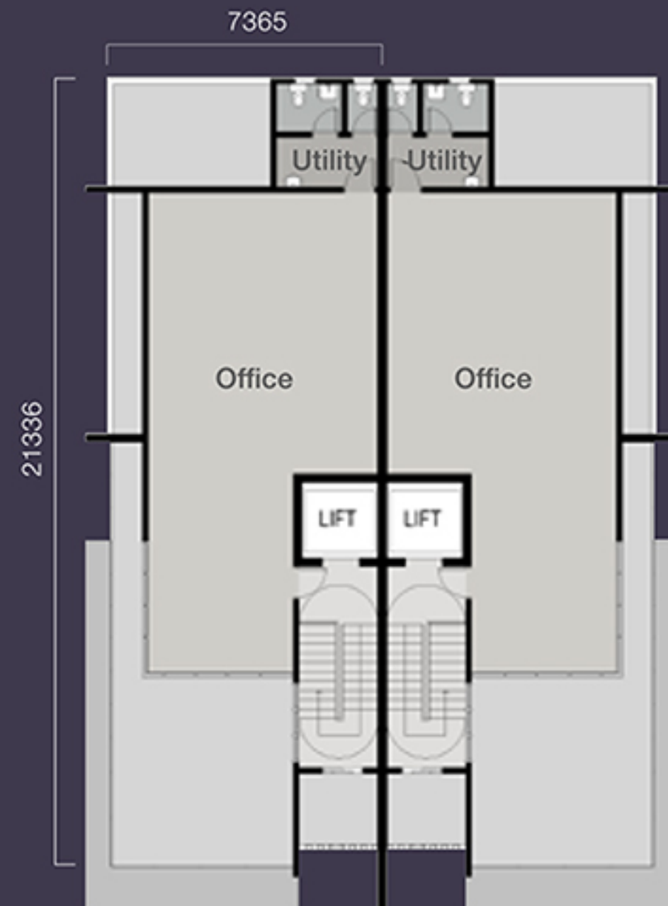
3rd Floor
