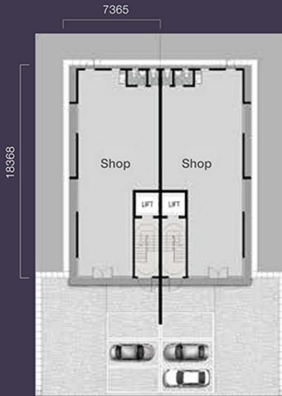
Ground Floor
