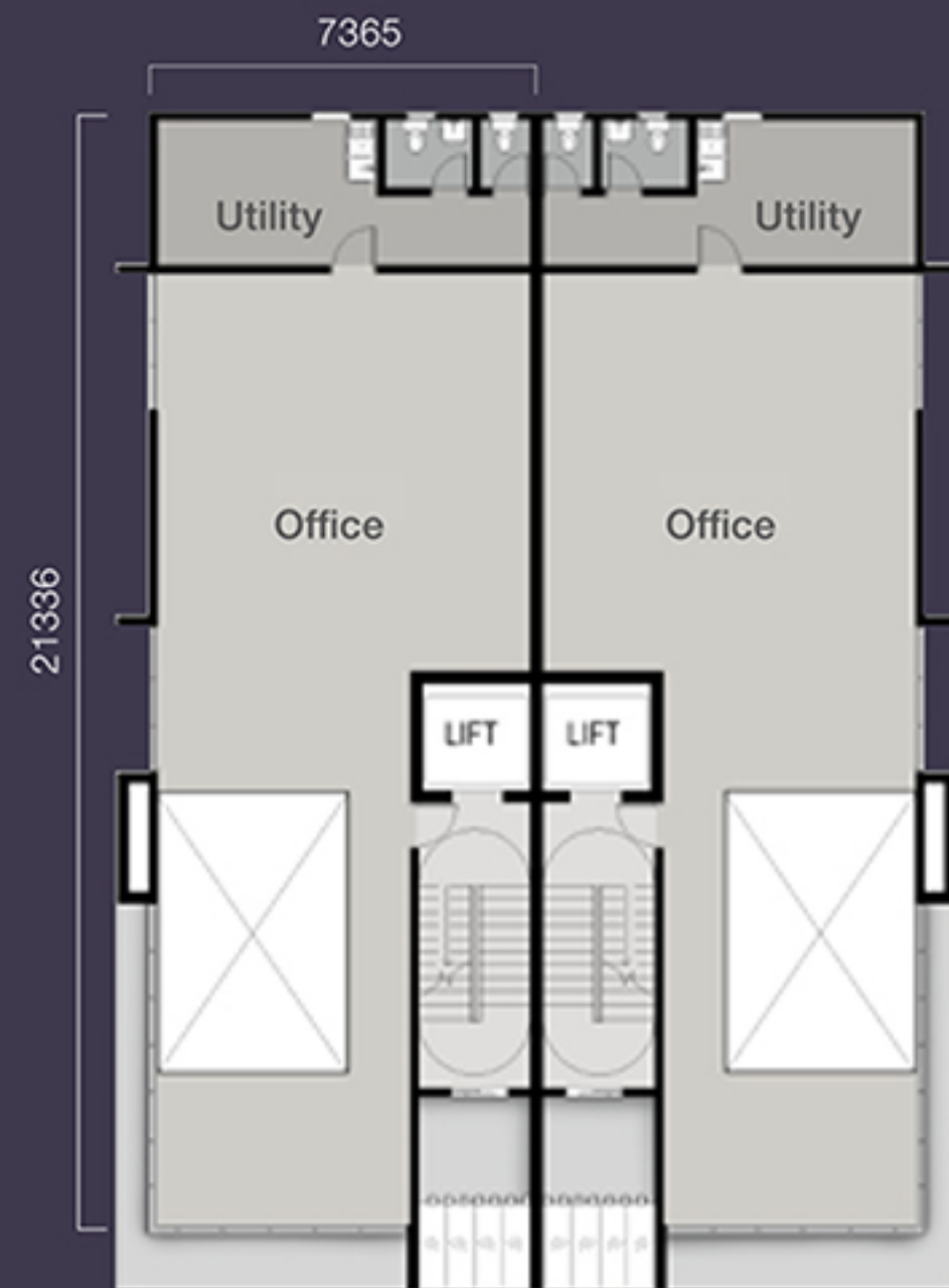
1st Floor
